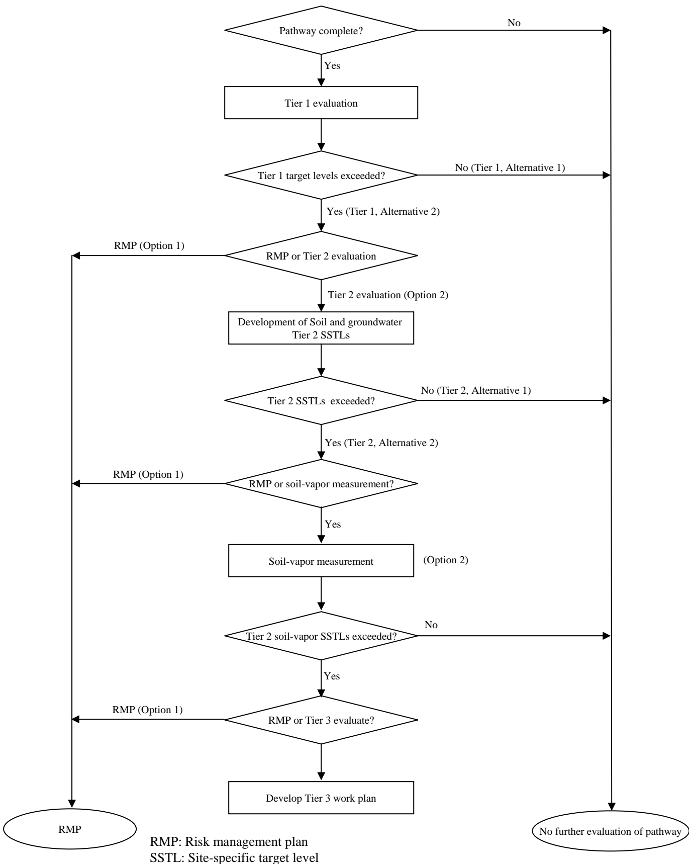
Figure C-1. Flowchart for Indoor Inhalation
