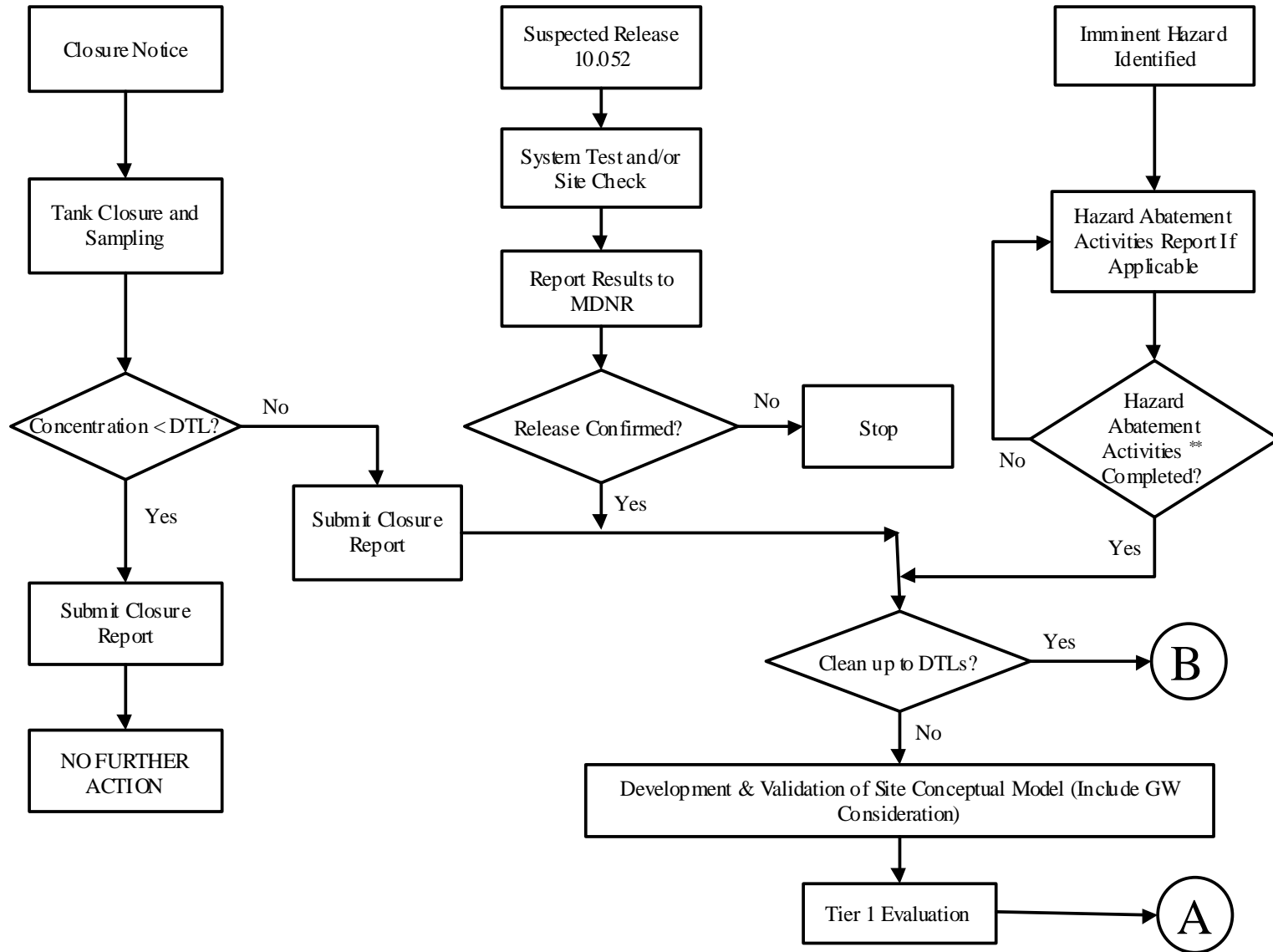
Figure 2-2. MRBCA Process Flowchart (Page 1 of 3)
